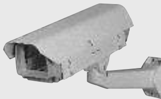
HHC12WM2 Box camera - 15" indoor/outdoor enclosure with mount, sunshield and 24VAC heater/blower
